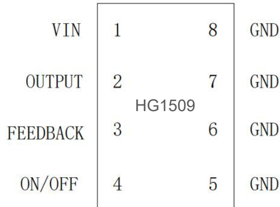
Figure1. Pin Configuration of HG1509 (Top View)
