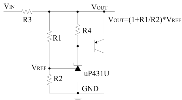
High Current Shunt Regulator
