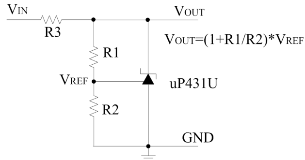
Shunt Regulator
