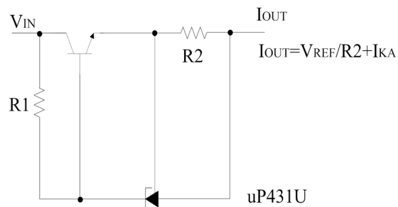
Current Source or Current Limit
