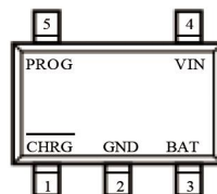
SOT-23-5L (TOP VIEW)
