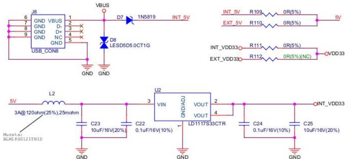
Fig. 5: ESP32-LCDKit Power Supply Module
