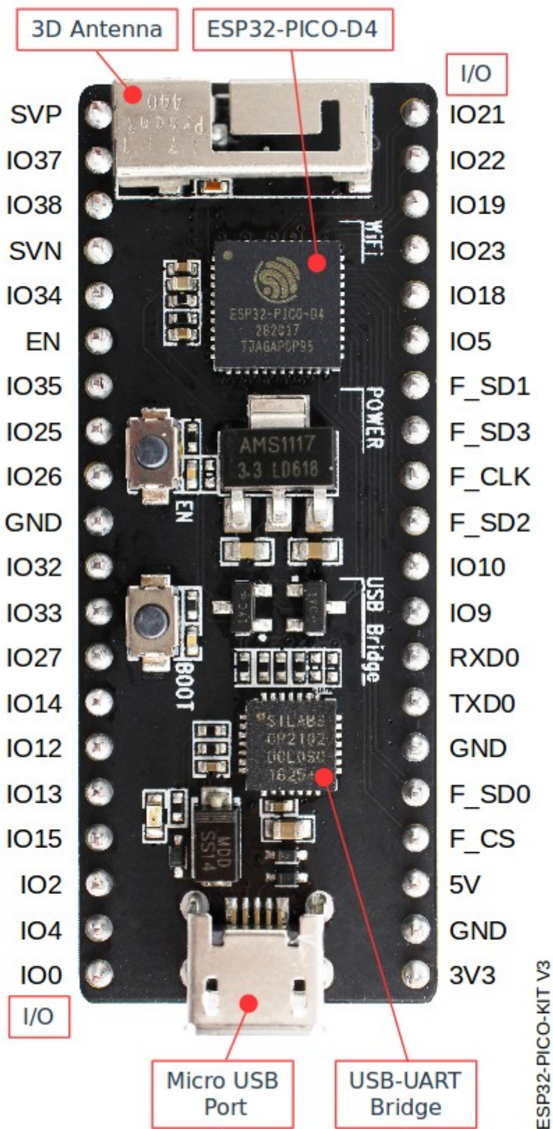
Fig. 38: ESP32-PICO-KIT v3 board layout (click to enlarge)
