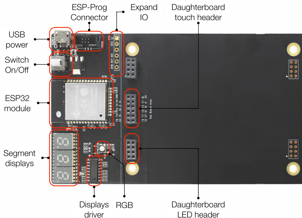
Fig. 8: Motherboard Components
