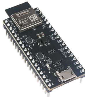
ESP32-PICO-DevKitM-2
