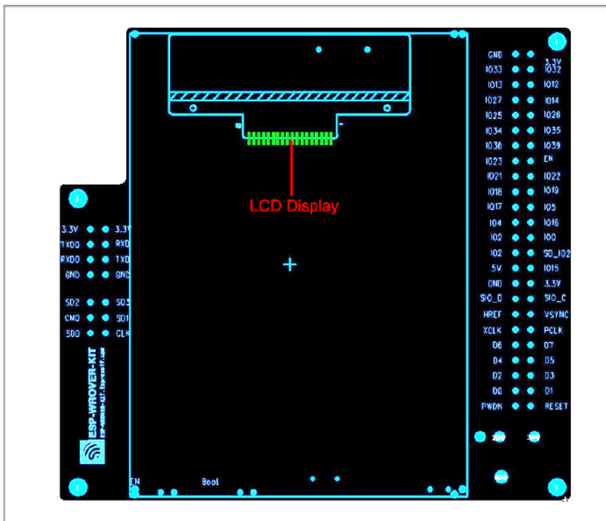
Fig. 28: ESP-WROVER-KIT board layout - back
