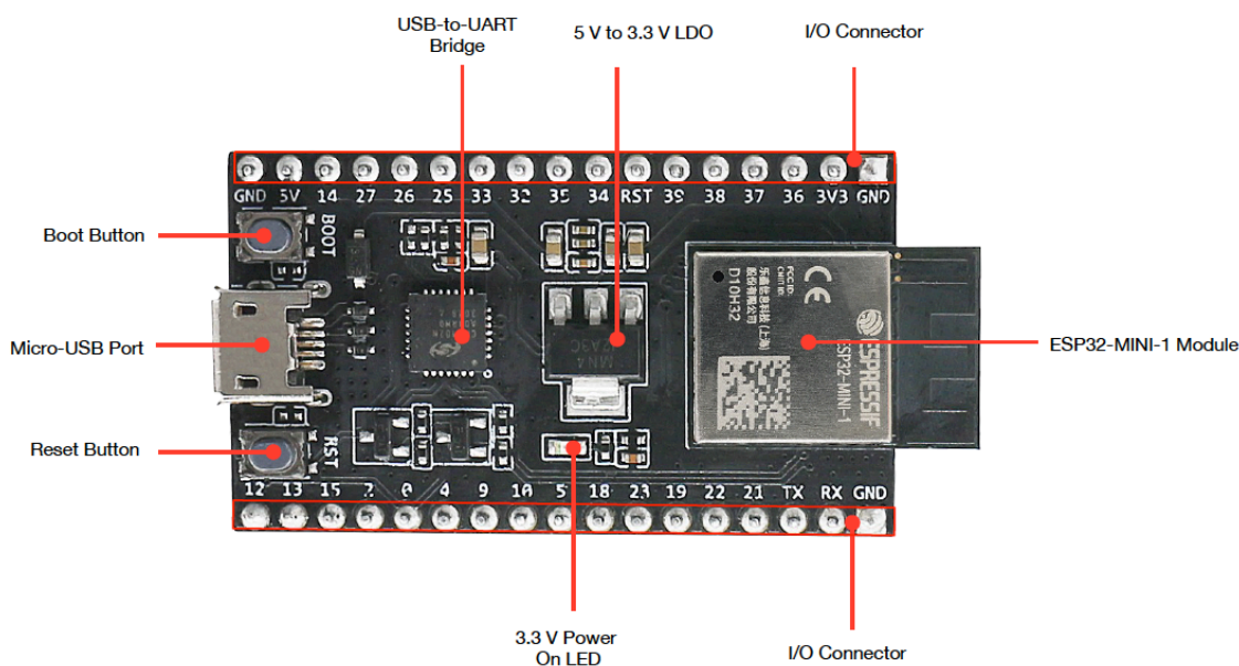
Fig. 1: ESP32-DevKitM-1 - front
