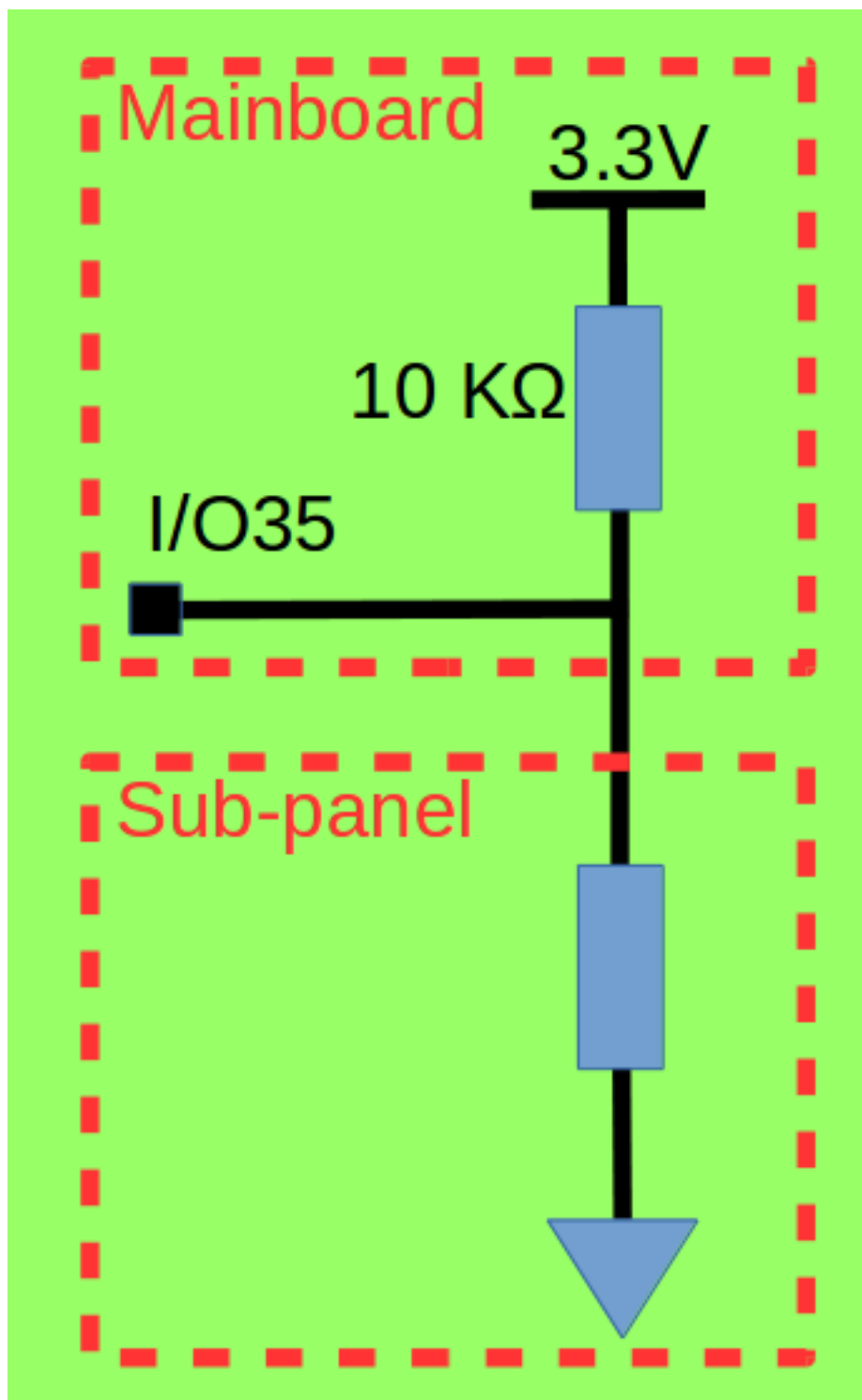
Fig. 11: Voltage Divider
