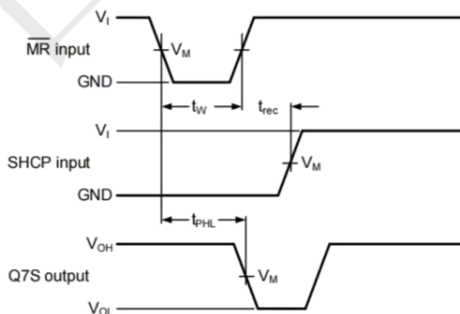
Figure 9. Master reset to output propagation delays
