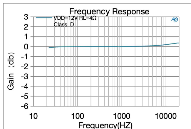
图 6: Frequency Response
