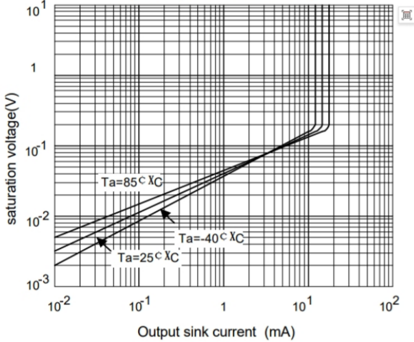
Fig.3 Output saturation voltage
