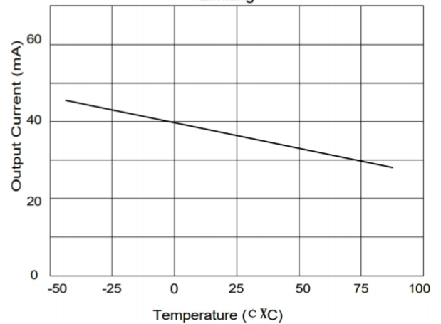
Fig.11 Current Limiting
