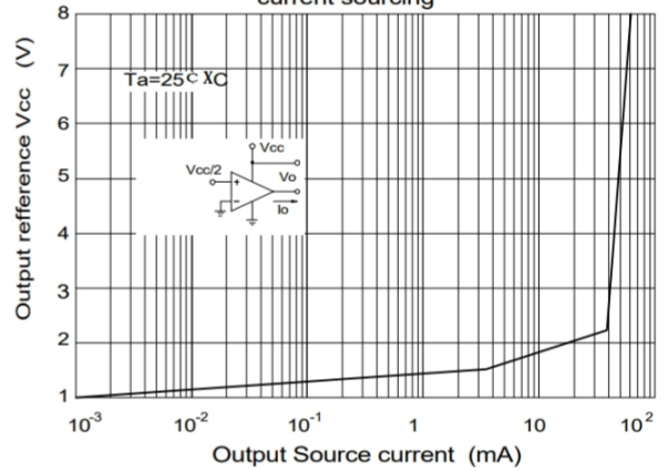
Fig.9 Output Characteristics current sourcing
