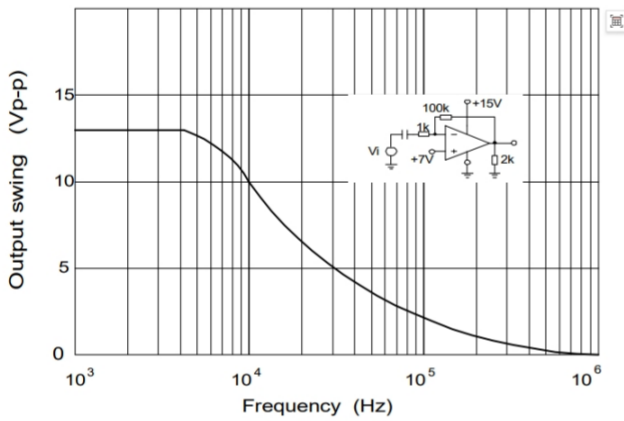
Fig.8 Large signal Frequency Response
