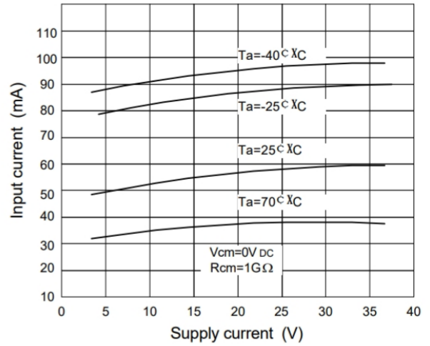
Fig.2 Input current
