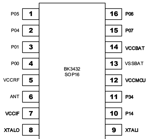
Figure 3 BK3432 SOP16 pin assignment
