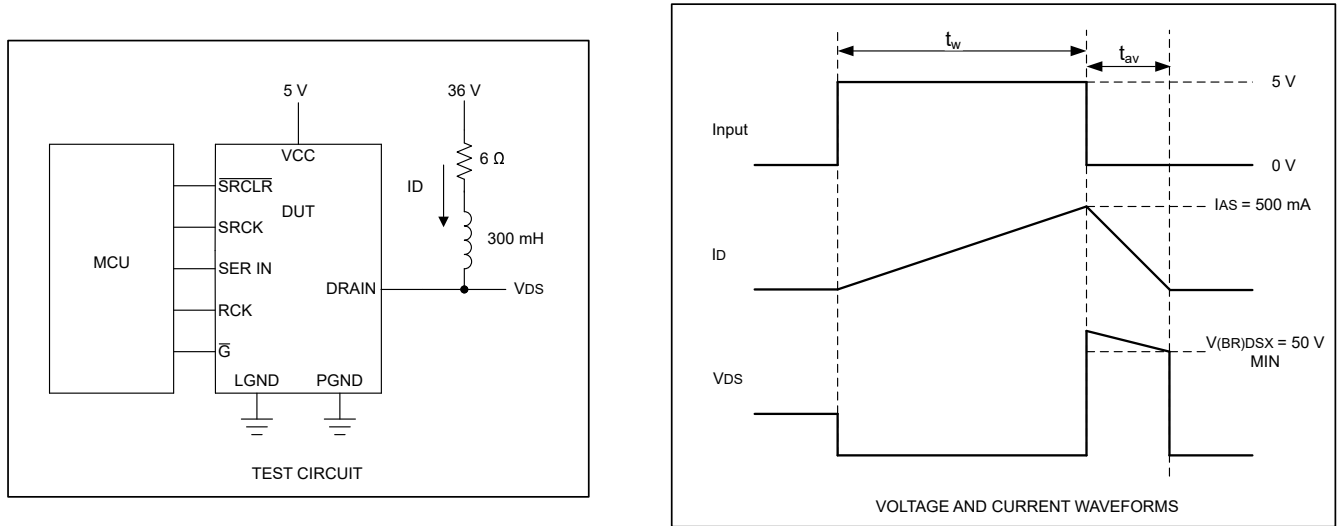
图 7-3. Single Pulse Avalanche Energy Test Circuit and Waveforms
