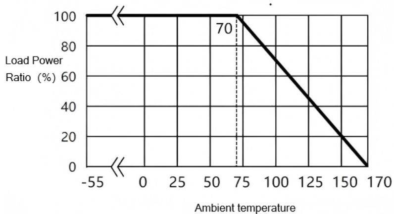
Power curve
