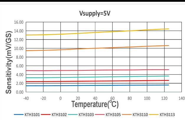
Sensitivity VS Temperature @VDD=5V
