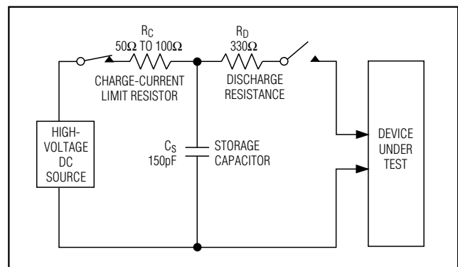
Figure 10. IEC 61000-4-2 Contact Discharge Test Model
