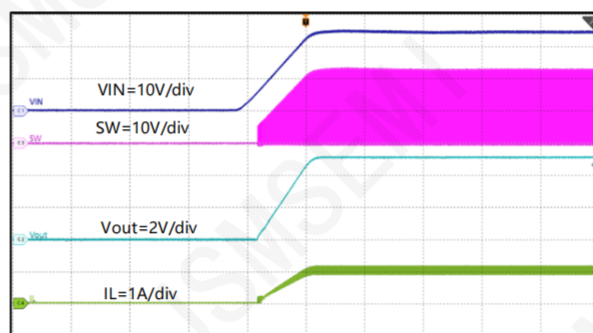
Figure 19. Start-Up with VIN Rising, I_{OUT}=1A
