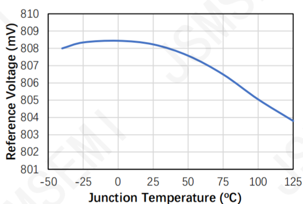
Figure 4. Reference Voltage vs. Junction Temperature
