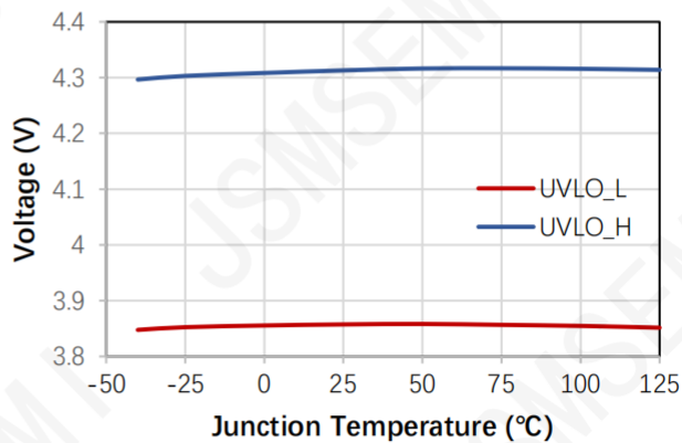
Figure 6. UVLO vs Junction Temperature
