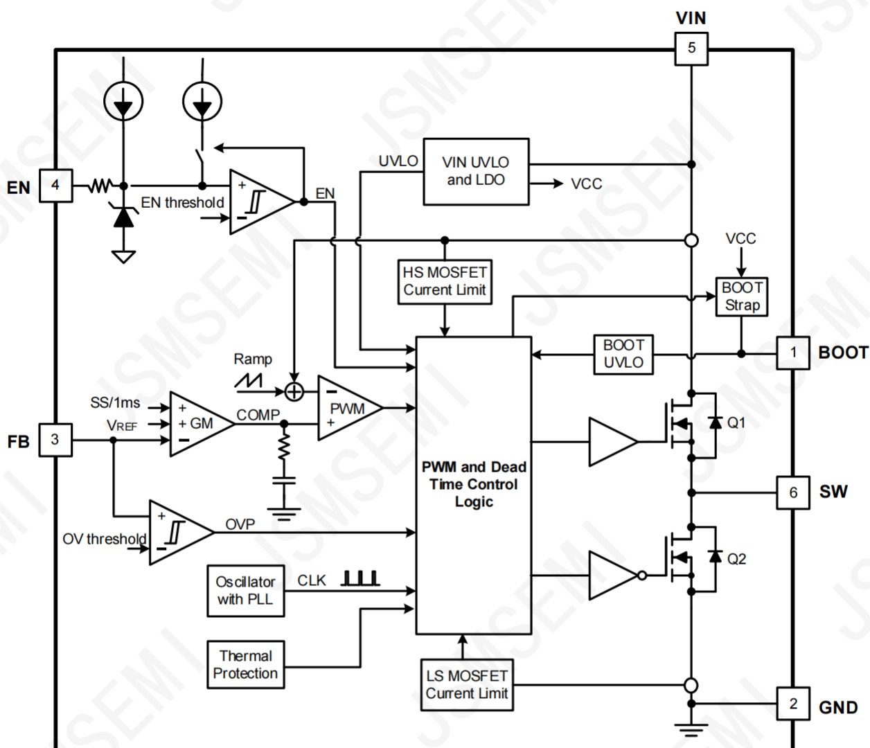
Figure 7. Block Diagram for LV2842YLVDDCR
