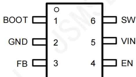
Top View: LV2842YLVDDCR TSOT23-6L
