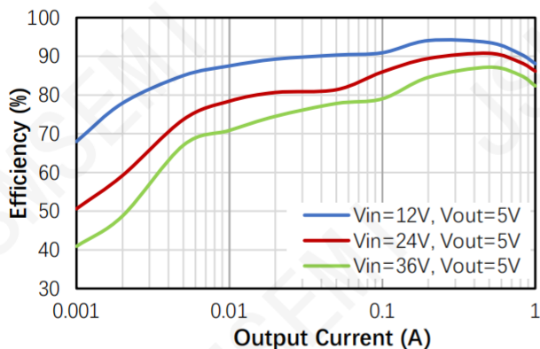
Figure 1. Efficiency Curve
