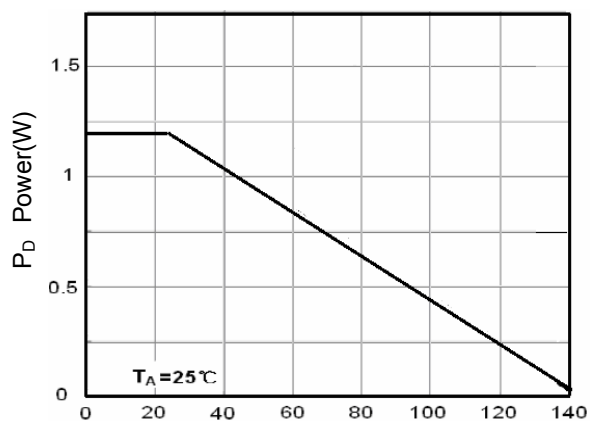
T_J -Junction Temperature( ^{\circ}C ) Figure 1 Power Dissipation
