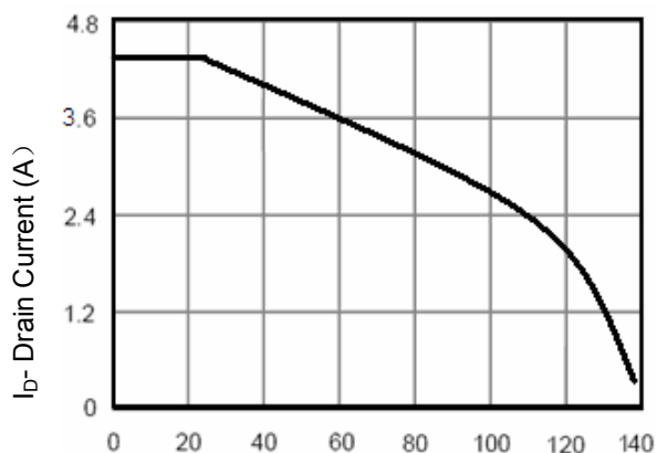
T_J -Junction Temperature( ^{\circ}C ) Figure 2 Drain Current
