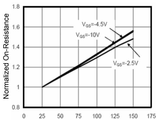
T_J -Junction Temperature( ^{\circ}C ) Figure 6 Drain-Source On-Resistance
