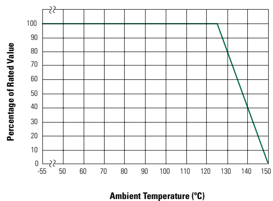
Figure 1B - Power Derating for Phenolic Coated
