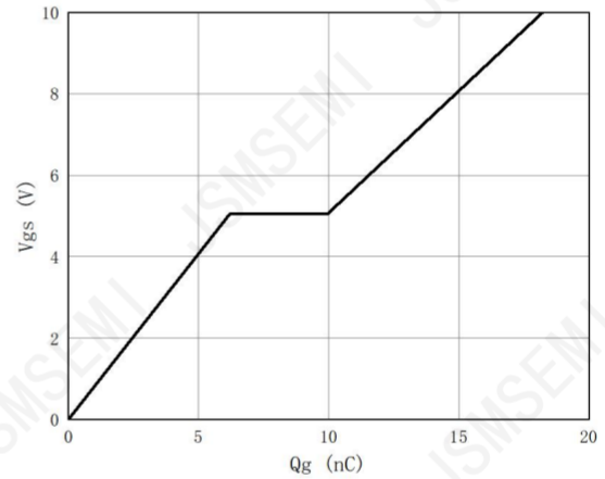
Figure 4. Gate-Charge Characteristics
