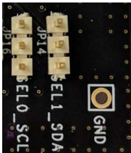
Figure 2. JP14 and JP16 Jumpers
