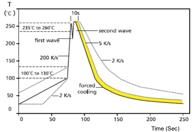
建議 double-wave Soldering Profile 實線：典型值 虛線：界限值
