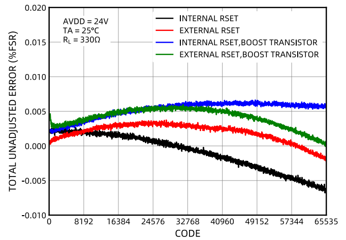
图 13 TUE vs DAC 码值
