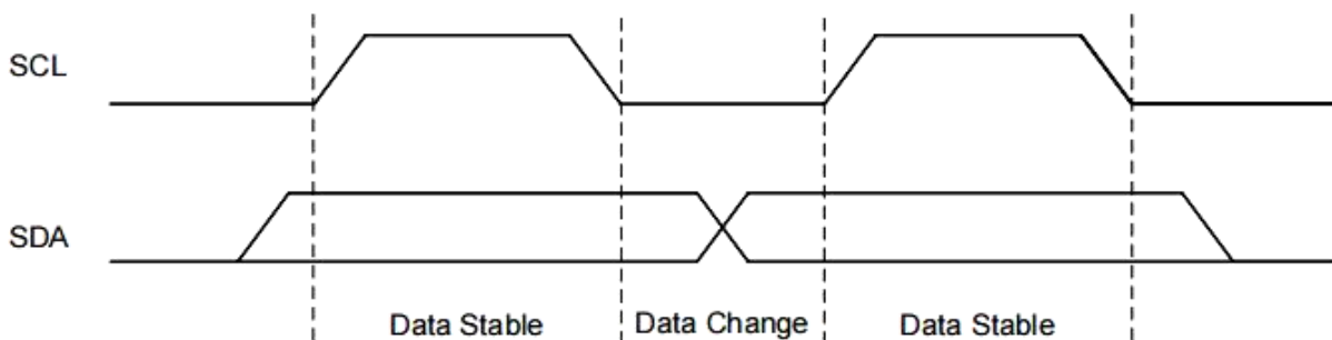
Figure 4-1 Data Validity
