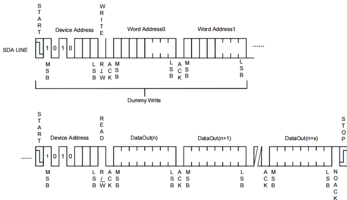
Figure 5-5 Sequential Read
