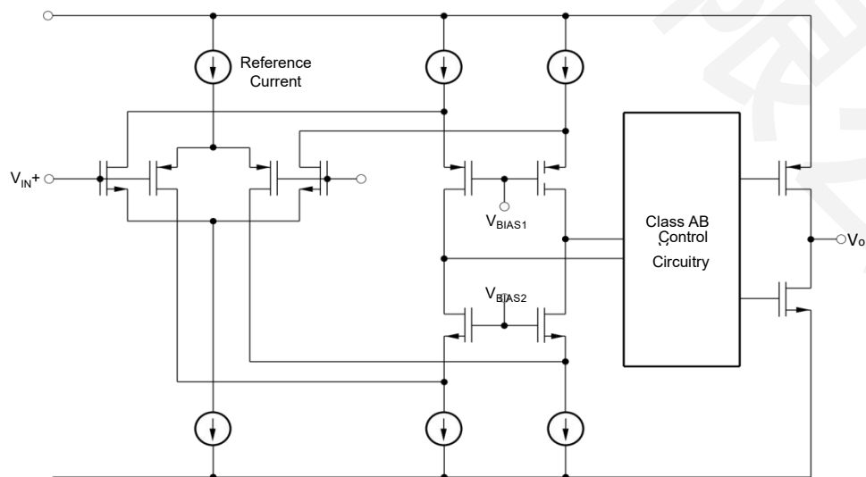
Figure 2. Simplified Schematic.
