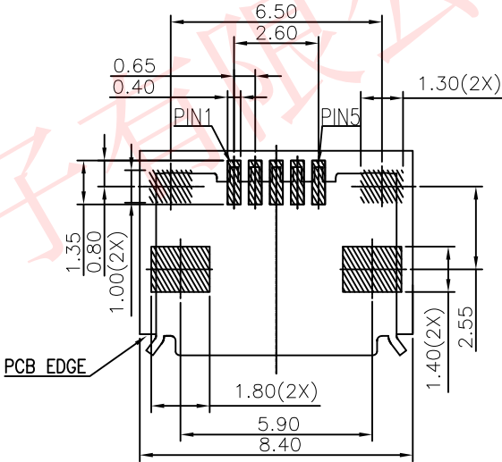
RECOMMENDED PCB LAYOUT(TOP VIEW) DEFAULT TOLERANCE:±0.05
