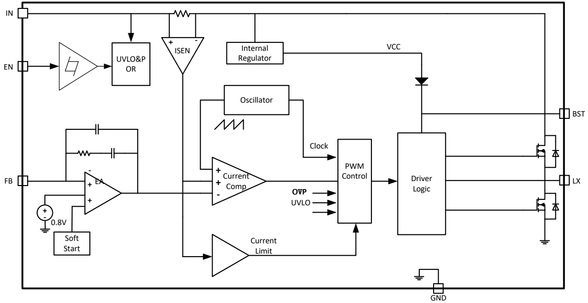
Figure 2. MSY8121BABC Block Diagram
