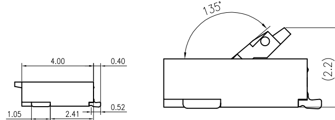
COVER OPEN STATE
