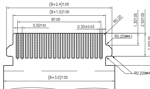
APPLICABLE FPC/FFC (THICKNESS 0.3±0.03)
