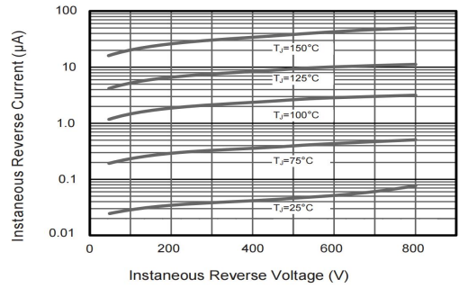
Fig.2 Typical Instaneous Reverse Characteristics
