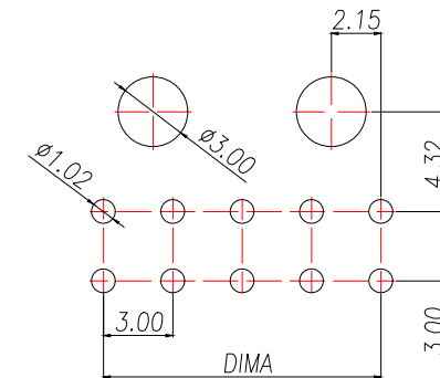
PCB.WELDING DRAWING (TOLERANCE:±0.05)
