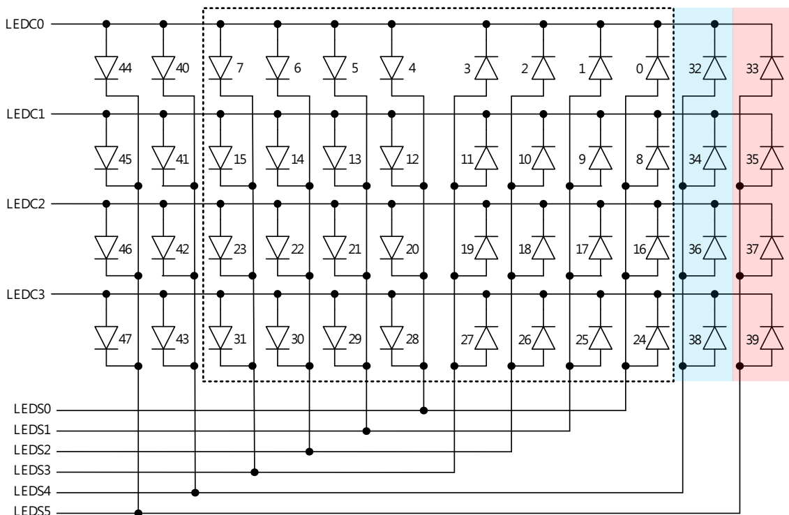
LED 4COM x 6SEG 正反扫模式对应像素点
