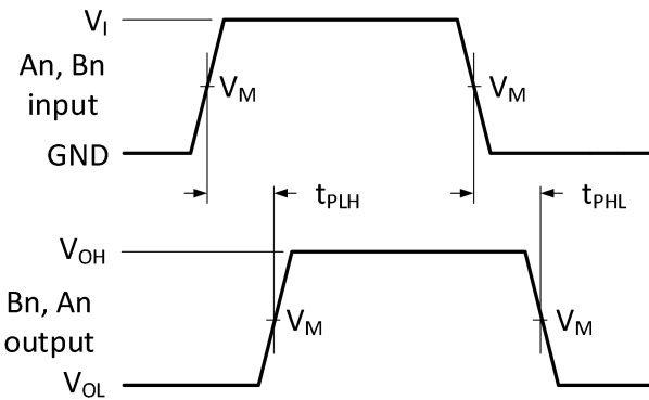
Measurement points are given in Table 8. V_{OL} and V_{OH} are typical output voltage levels that occur with the output load.
