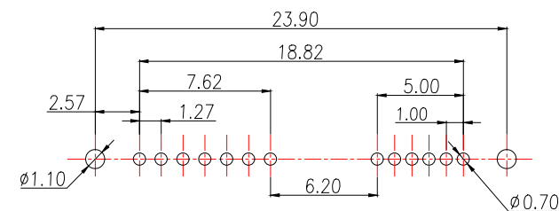
PCB LAYOUT
