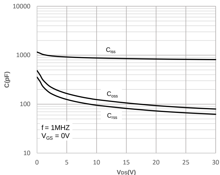
Figure 6: Capacitance Characteristics
