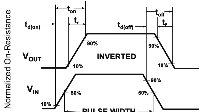
Figure 2: Switching Waveforms
