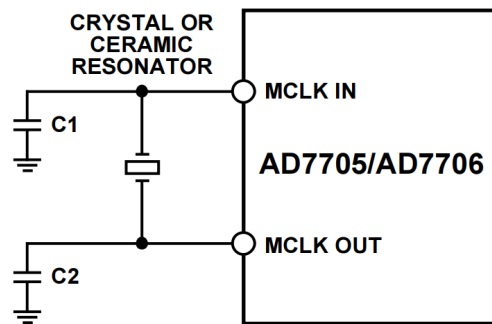
Figure 7. Crystal/Resonator Connection for the AD7705/AD7706
