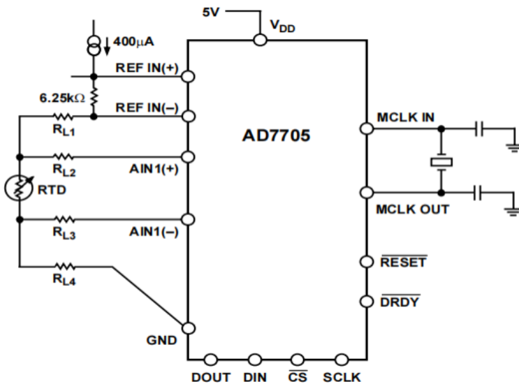
Figure 16. Temperature Measurement Using the AD7705
