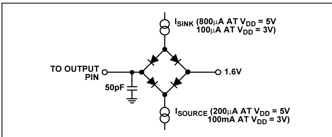
Figure 2. Load Circuit for Access Time and Bus Relinquish Time
