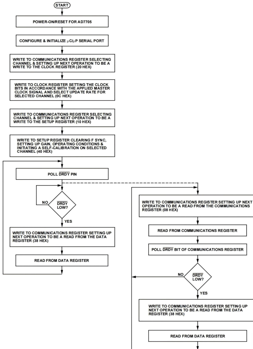
Figure 11. Flowchart for Setting Up and Reading from the AD7705
