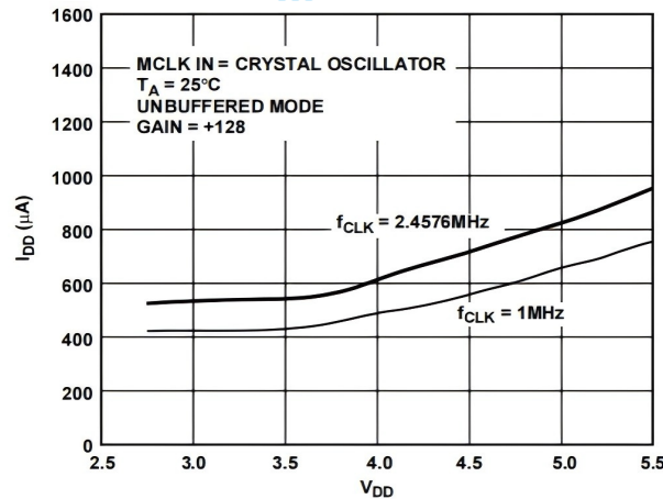
Figure 8. I DD vs. Supply Voltage
