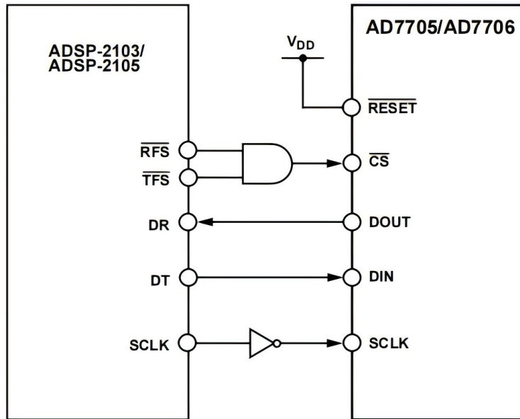
Figure 14. AD7705/AD7706-to-ADSP-2103/ADSP-2105 Interface
