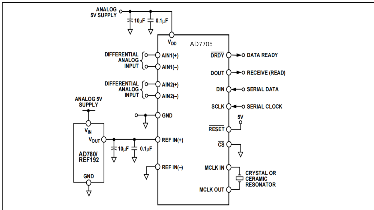
Figure 3. AD7705 Basic Connection Diagram
