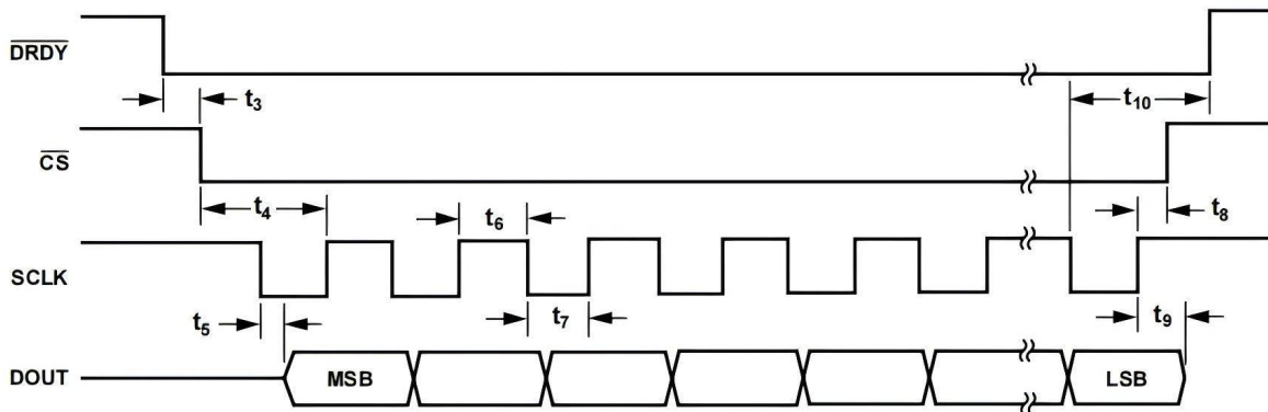
Figure 9. Read Cycle Timing Diagram
