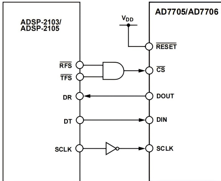
Figure 14. AD7705/AD7706-to-ADSP-2103/ADSP-2105 Interface
