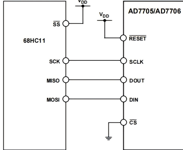
Figure 12.AD7705/AD7706-to-68HC11 Interface
