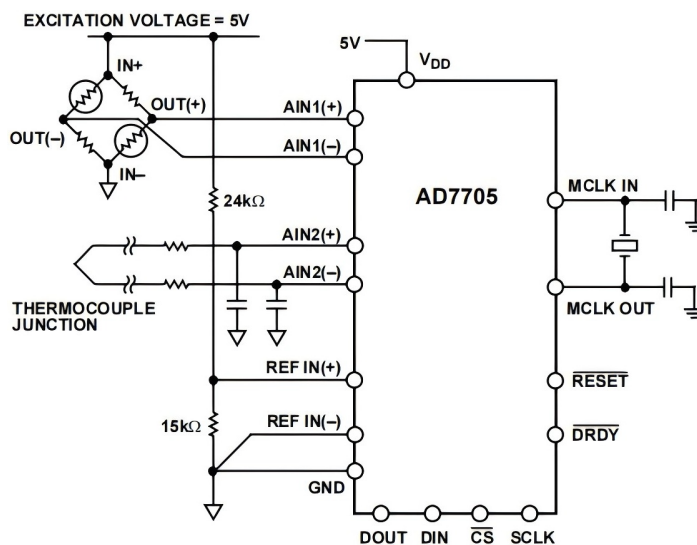
Figure 15. Pressure Measurement Using the AD7705
