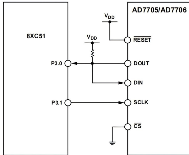
Figure 13.AD7705/AD7706-to-8XC51 Interface
