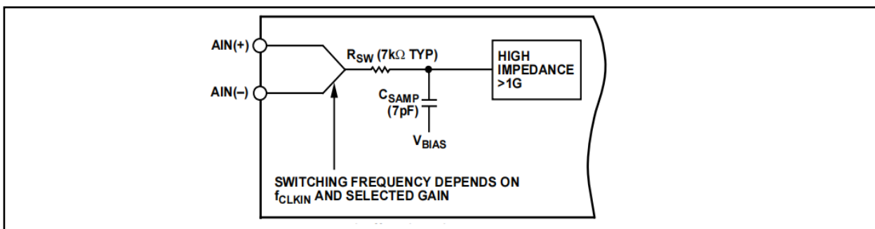
Figure 4. Unbuffered Analog Input Structure
