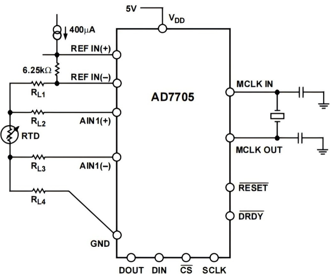
Figure 27. RTD Measurement Using the AD7705
