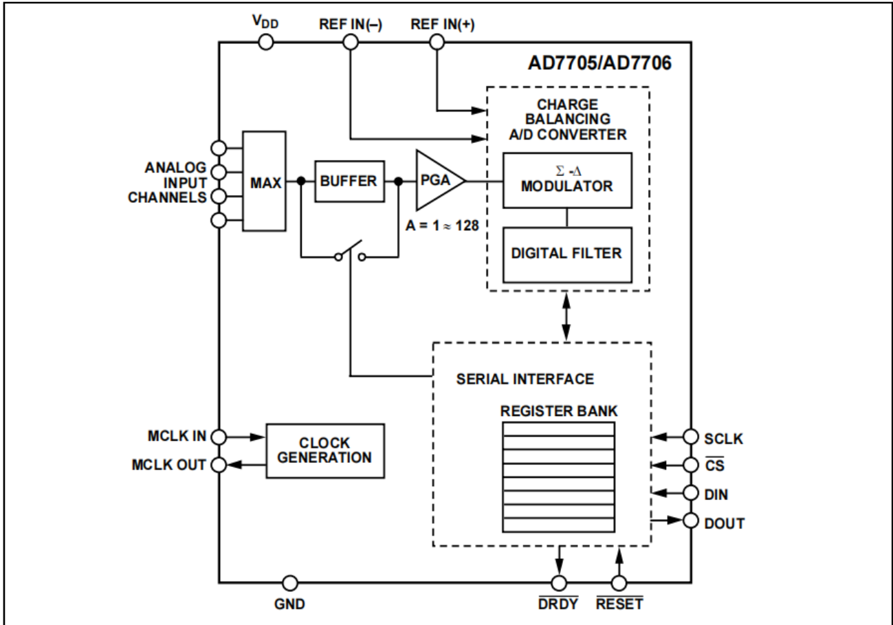
Figure 1. AD7705/7706 Functional block diagram
