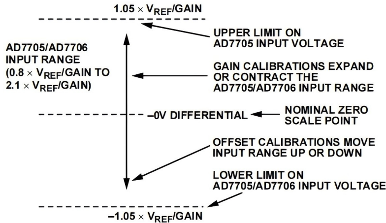
Figure 6. Span and Offset Limits
