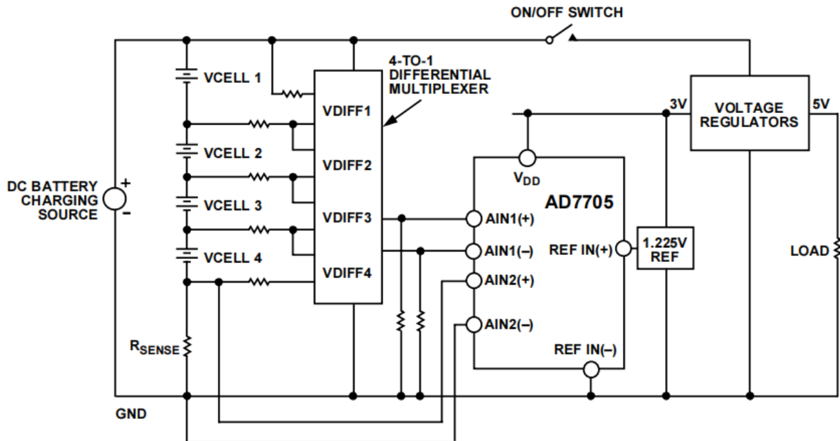
Figure 19. Battery Monitoring Using the AD7705
