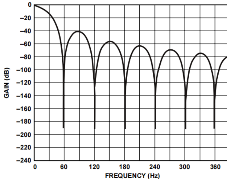
Figure 5. Frequency Response of AD7705 Filter
