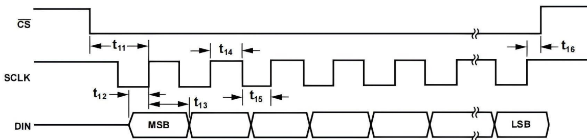
Figure 20. Write Cycle Timing Diagram
