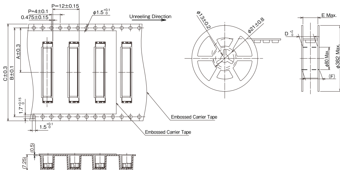
Embossed Carrier Tape Dimensions (No scale)
