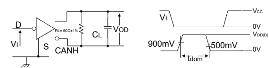
F10. Revealed Timeout Test Circuit and Waveforms
