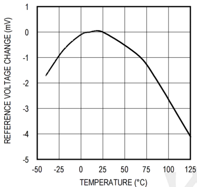
TEMPERATURE DRIFT
