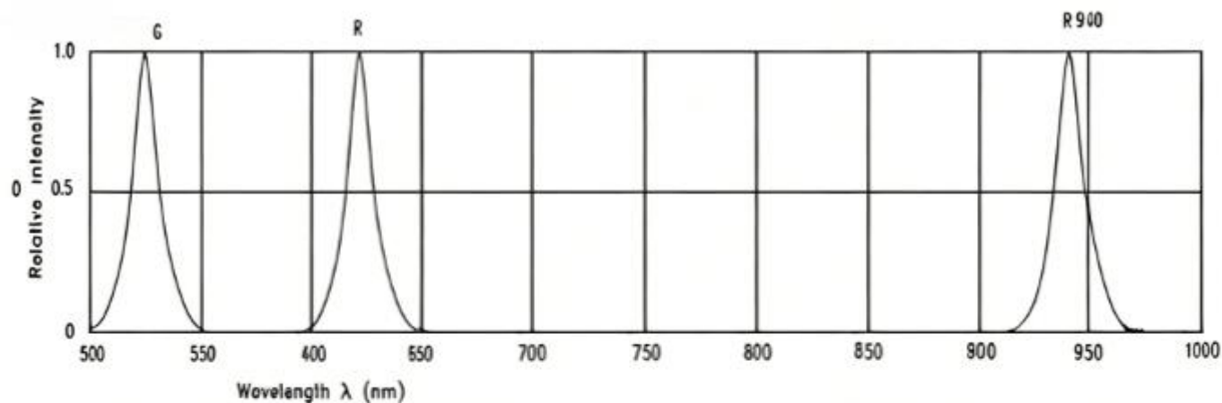
Fig.1 RELATIVE INTENSITY VS. WAVELENGTH
