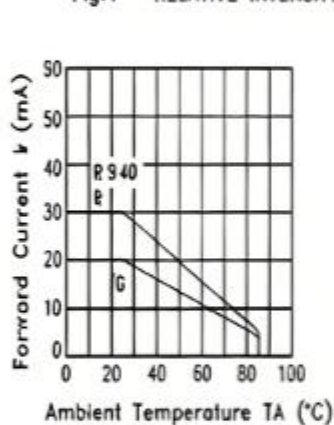
Fig.3 FORWARD CURRENT DERATING CURVE
