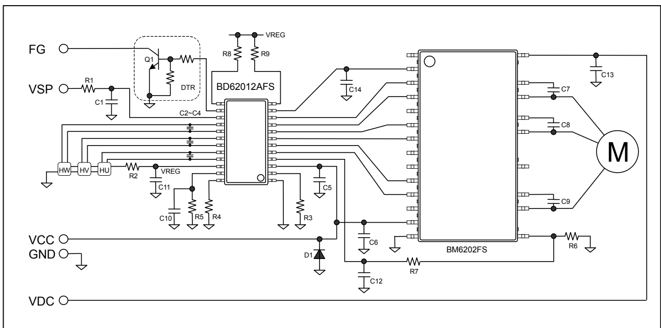
Figure 1. Application circuit example - BD62012AFS & BM6202FS
