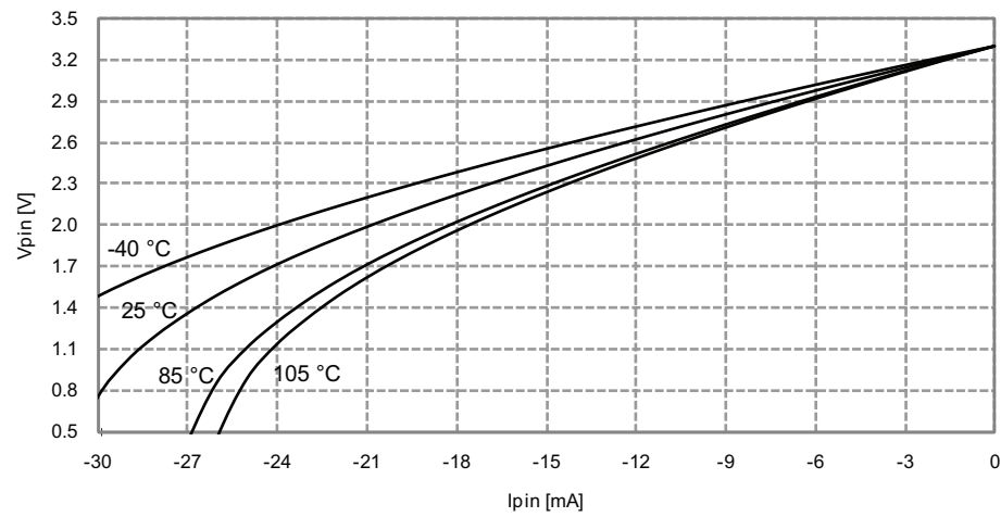
Figure 33-268. I/O Pin Output Voltage vs. Source Current
