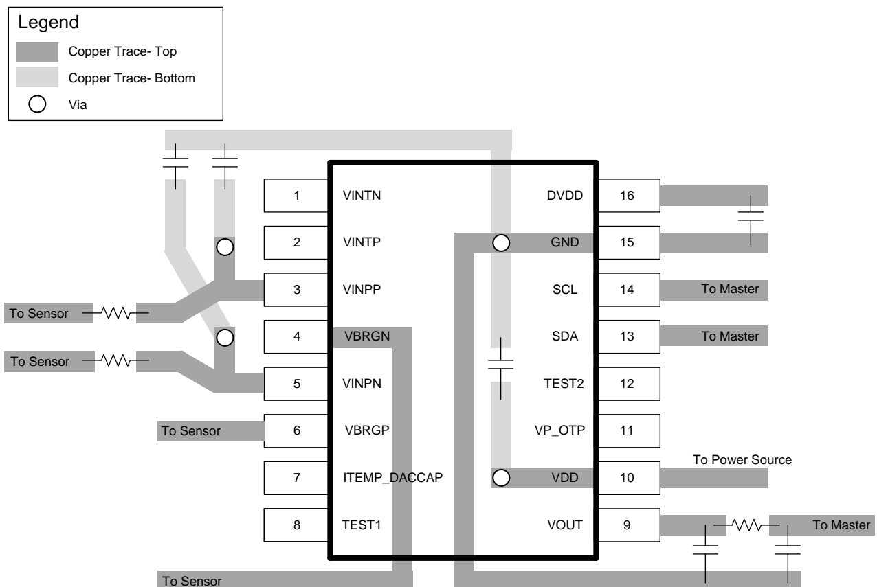
Figure 118. Layout Example
