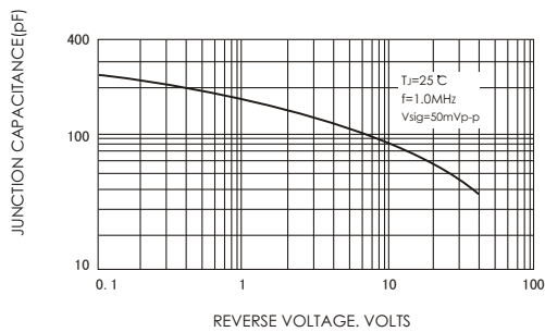
FIG.5-TYPICAL JUNCTION CAPACITANCE
