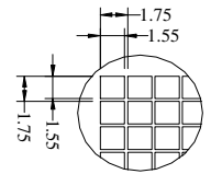
Detail "A" Scale (10:1)
