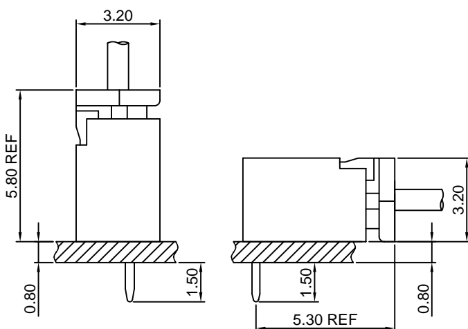
DIP TYPE
