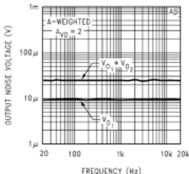
Noise Floor
