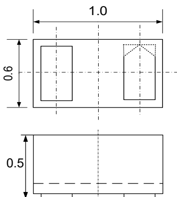
Package Dimensions
