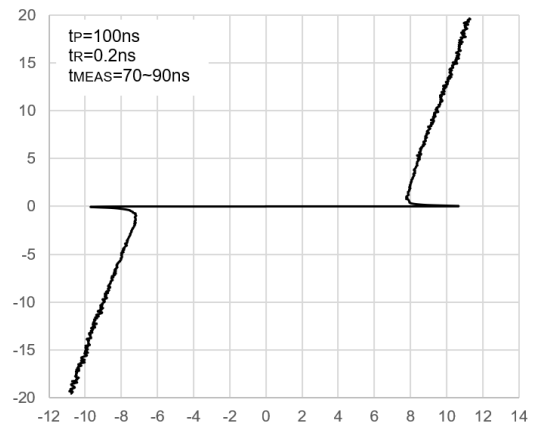
TLP IV Curve
