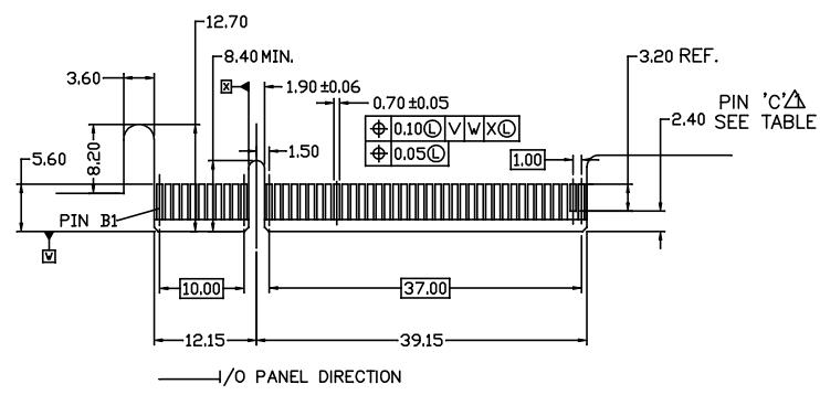
PRIMARY (COMPONENT) SIDE
