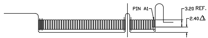
SECONDARY (SOLDER) SIDE
