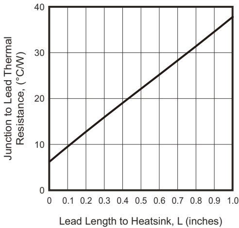
Fig.3 - Typical Thermal Resistance v.s. Lead Length
