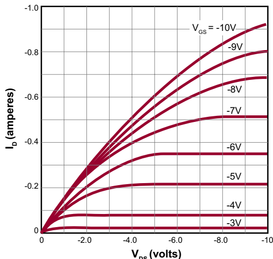
Saturation Characteristics
