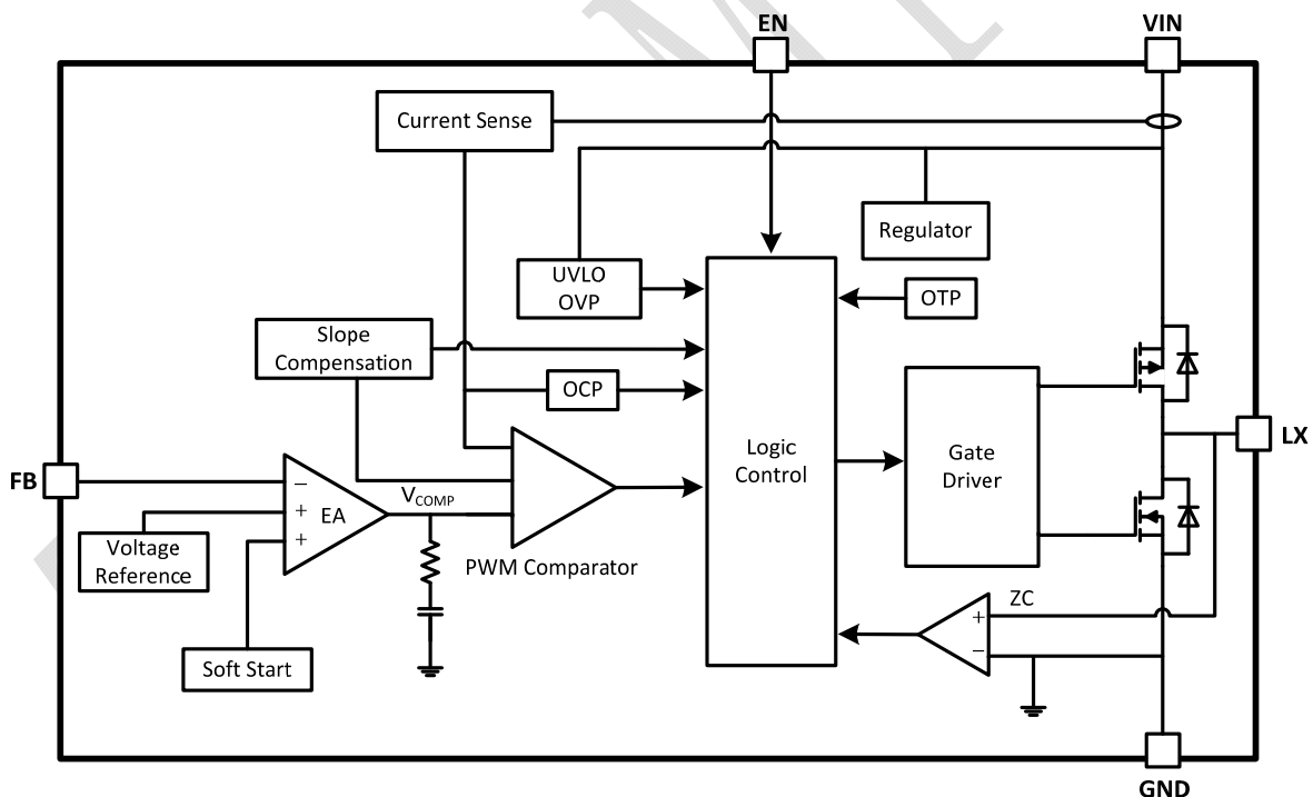
Figure 3. TMI3411 Block Diagram
