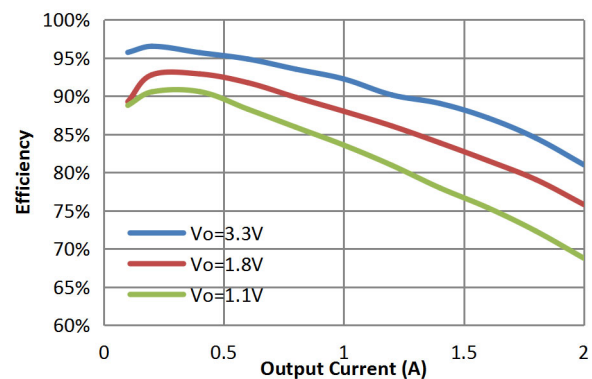
Figure 2. Efficiency ( V_{IN}=5V , I_o=0.1A to 2A )
