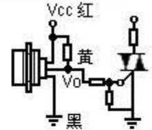
NPN型接双向可控硅
