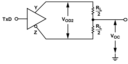
Figure 23. Driver Voltage Measurement
